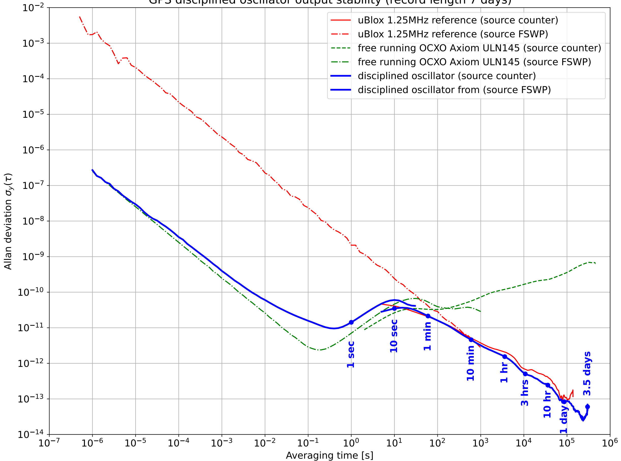
GPS disciplined oscillator output stability (record length 7 days)
