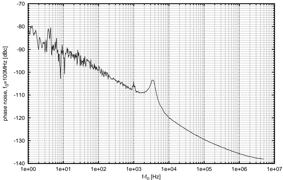
SNM PDC delay line / phase stepper preliminary phase noise measurement ( f_0=100\text{MHz} , 3V3 LVCMOS into 50\Omega , without galvanic isolation)
